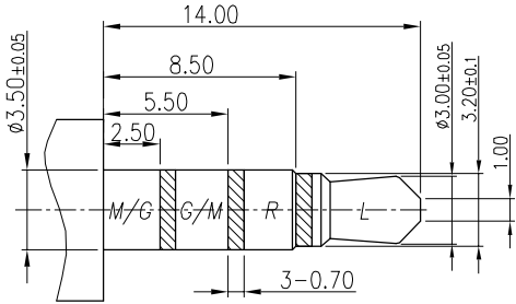
RECOMMENDED PLUG; TOL. ±0.05 ø3.5 4-POLE PLUG
