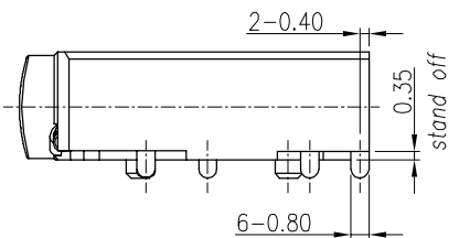
RECOMMENDED PLUG; TOL. ±0.05 ø3.5 4-POLE PLUG
