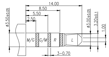
RECOMMENDED PLUG(±0.05) ø3.5 4-POLE STANDARD PLUG
