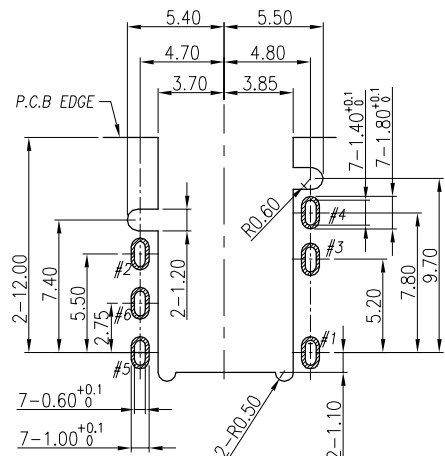
RECOMMENDED PCB LAYOUT TOP VIEW ; TOL.±0.05
