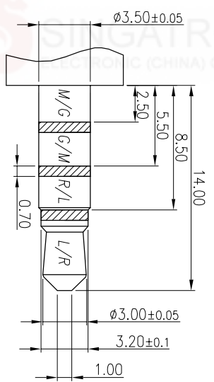
RECOMMENDED PLUG Ø3.5 4-POLE STANDARD PLUG
