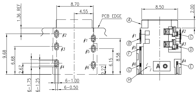
RECOMMENDED PCB LAYOUT TOP VIEW ; TOL.±0.05
