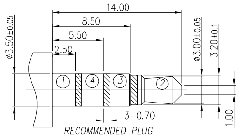
ø3.5 4-POLE STANDARD PLUG
