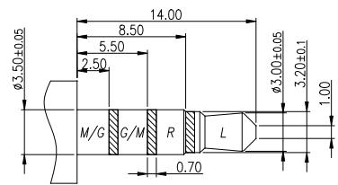
RECOMMENDED PLUG Ø3.5 4-POLE PLUG(TOL.±0.05)
