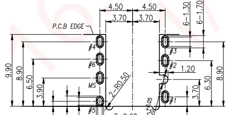
RECOMMENDED PCB LAYOUT TOP VIEW ; TOL.±0.05
