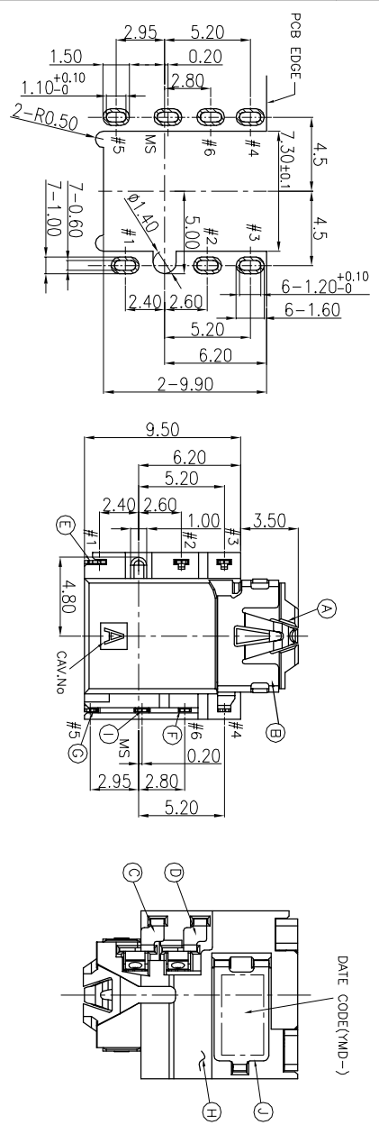
RECOMMENDED PCB LAYOUT(TOP VIEW) TOP VIEW: TOL.±0.05
