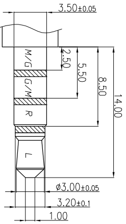
RECOMMENDED PLUG Ø3.5 4-POLE STANDARD PLUG
