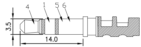
Ø3.5 MATE PLUG
