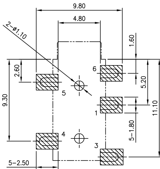
RECOMMENDED PADS LAYOUT <TOP VIEW>
