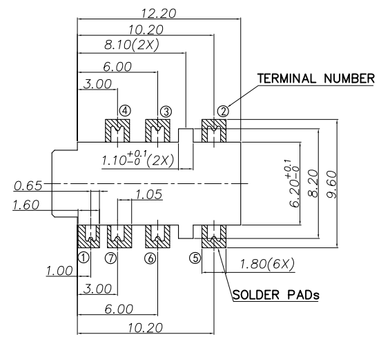
PCB LAYOUT (TOP VIEW) TOLERANCE: ±0.05mm
