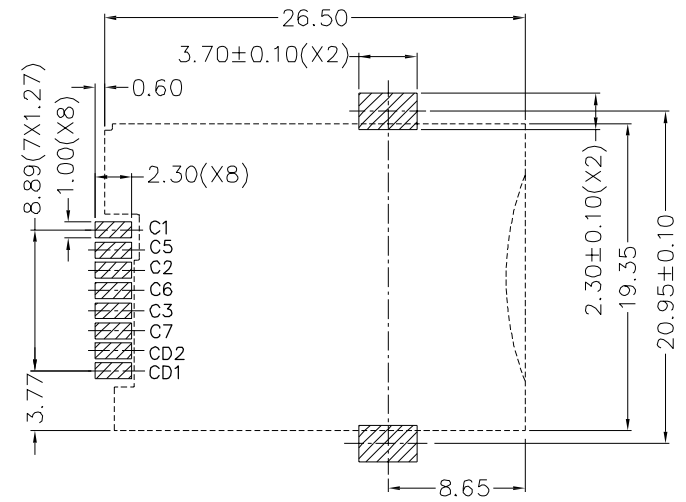
RECOMMENDED P.C.B LAYOUT COMPONENT SIDE (TOLERANCE ±0.05)
