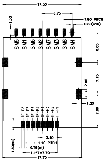
RECOMMENDED PCB LAYOUT TOLERANCE=±0.05
