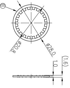
SPRING WASHER
