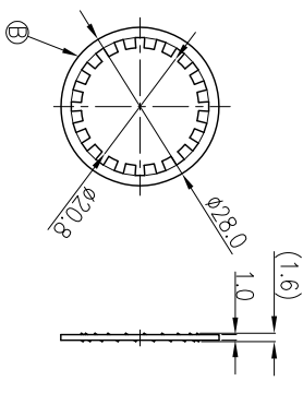
SPRING WASHER (1.6)
