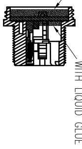
CONN.1 WATERPROOF RATE: IP67
