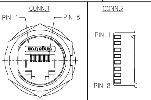
PIN ASSIGNMENTS FRONT VIEW
