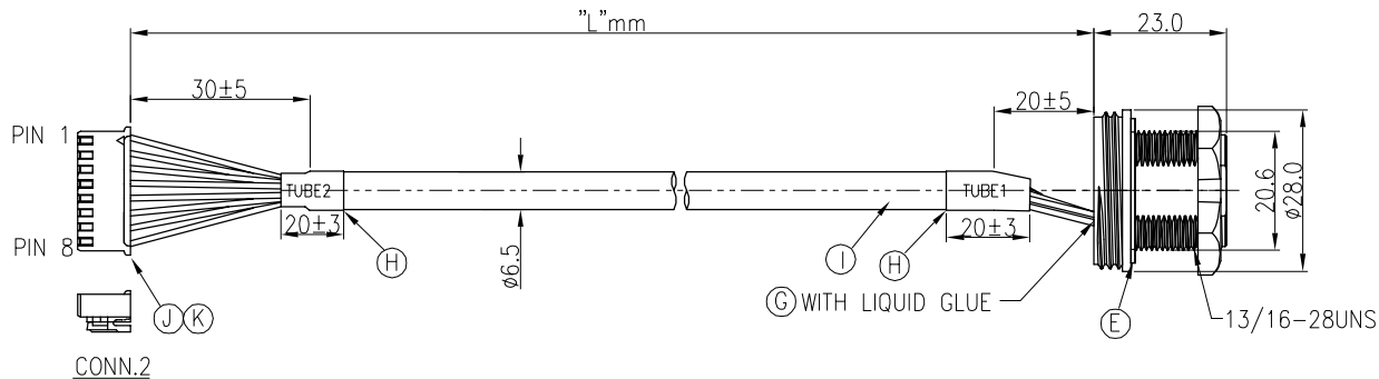
CONN.1 WATERPROOF RATE: IP67
