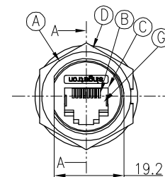
CONN.1 WATERPROOF RATE: IP67
