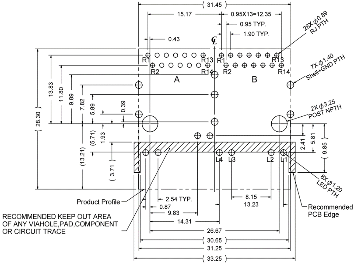
RECOMMENDED PCB LAYOUT ALL DIMENSION TOLERANCES ARE \pm 0.05 mm UNLESS OTHERWISE SPECIFIED
