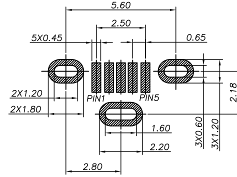
RECOMMENDED PCB LAYOUT(TOP VIEW) GENERAL TOLERANCES:±0.05
