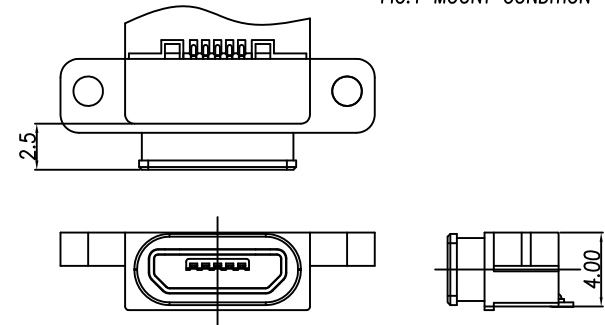
FIG.1 MOUNT CONDITION
