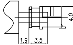
FIG.2 MATING CONDITION
