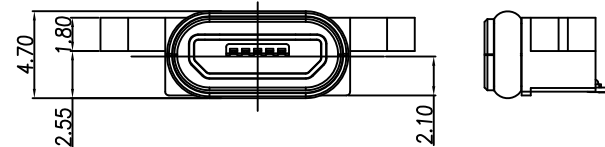
FIG.3 GASKET INTEGRATION CONDITION
