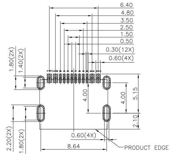
RECOMMENDED PCB LAYOUT(TOP VIEW) THICKNESS 0.60MM;DEFAULT TOLERANCE:±0.05
