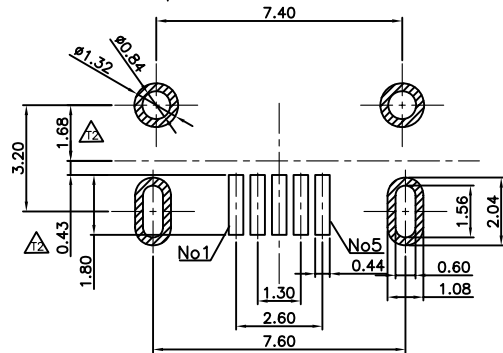
RECOMMENDED PCB LAYOUT TOLERANCE: ±0.03mm RECOMMEND PCB THICKNESS: 0.80mm
