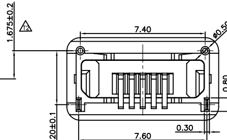
ASSEMBLY WITH CAP
