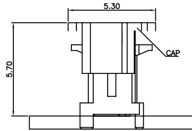
ASSEMBLY WITH CAP
