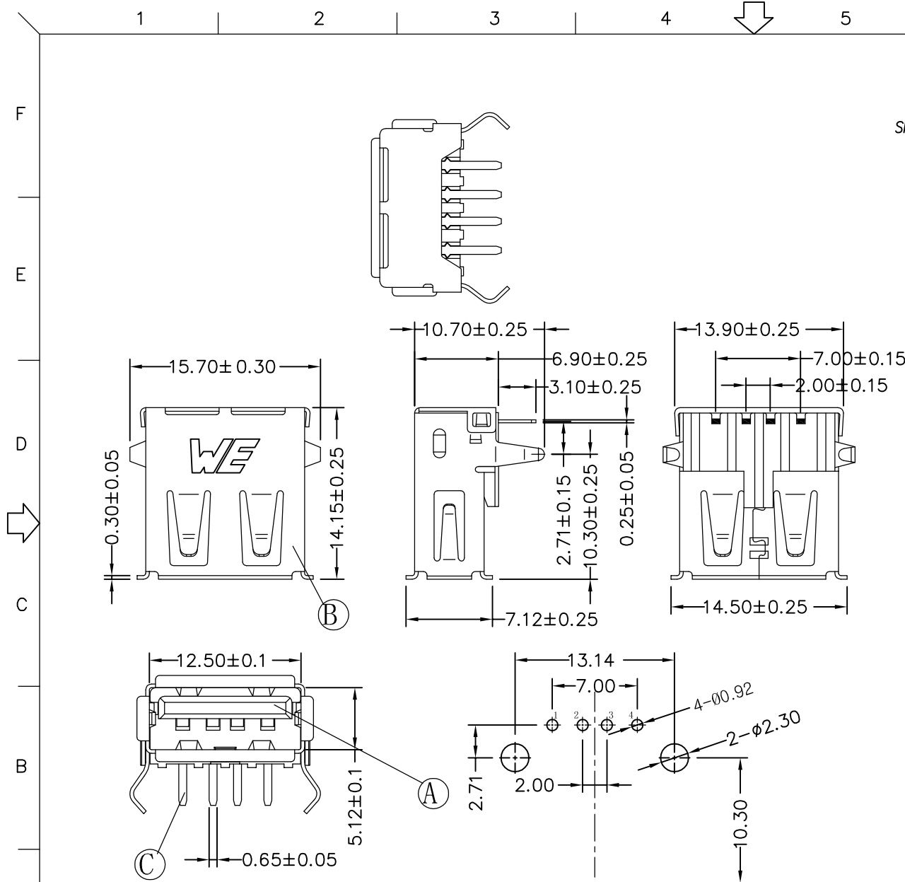
RECOMMENDED P.C.B. PATTERN LAYOUT
