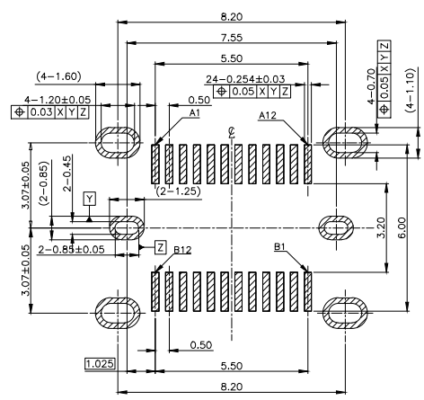
RECOMMENDED PCB LAYOUT TOP VIEW SCALE 2:1 (TOLERANCE=±0.05mm)
