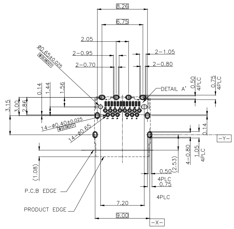
RECOMMENDED P.C.B LAYOUT(TOP VIEW) TOLERANCE=±0.05(THK:1.6mm)
