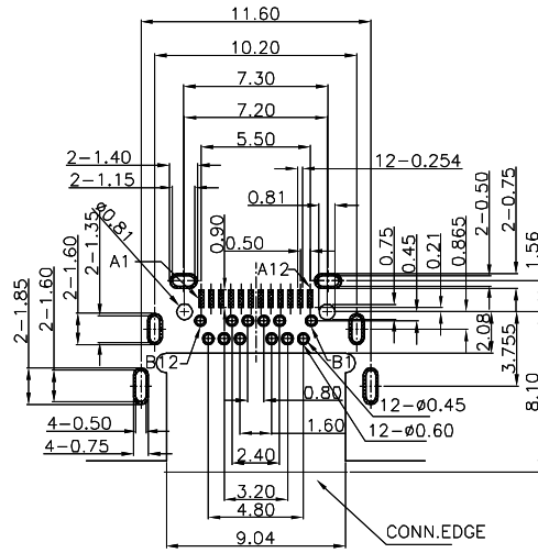
RECOMMENDED P.C.B LAYOUT(TOP VIEW) TOLERANCE=±0.05(THK:1.00mm)
