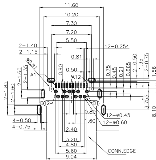
RECOMMENDED P.C.B LAYOUT(TOP VIEW) TOLERANCE=±0.05(THK: 1.00mm)
