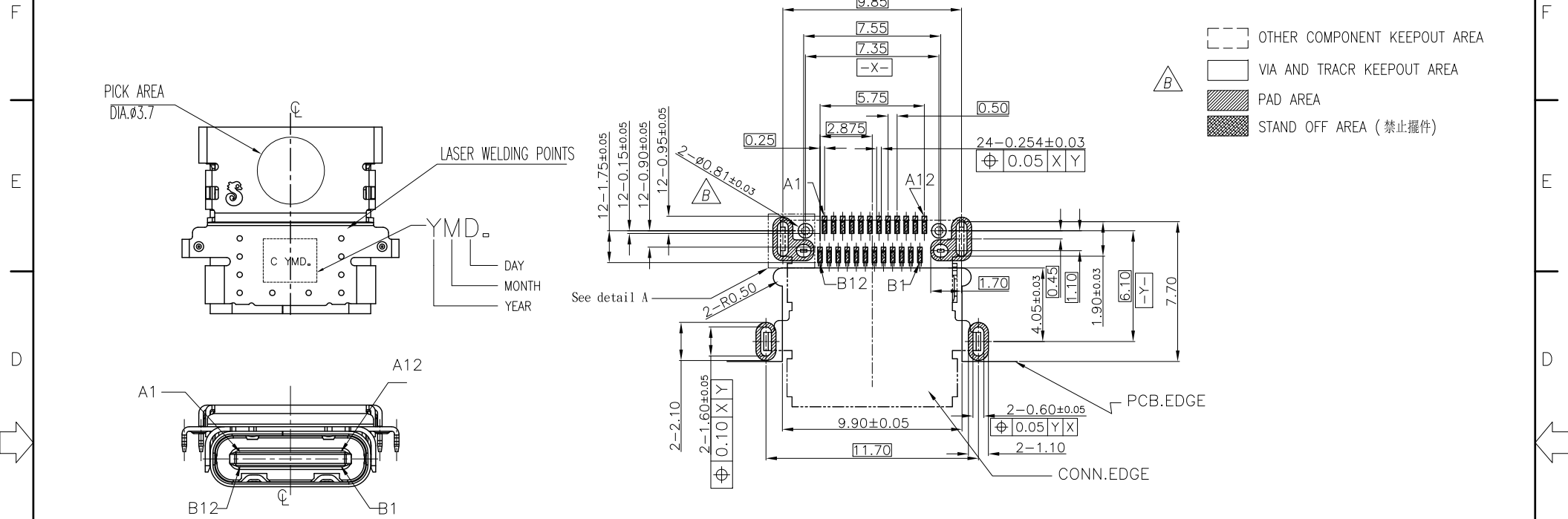
RECOMMENDED P.C.B LAYOUT(TOP VIEW) TOLERANCE = \pm 0.05 (THK: 1.00mm)
