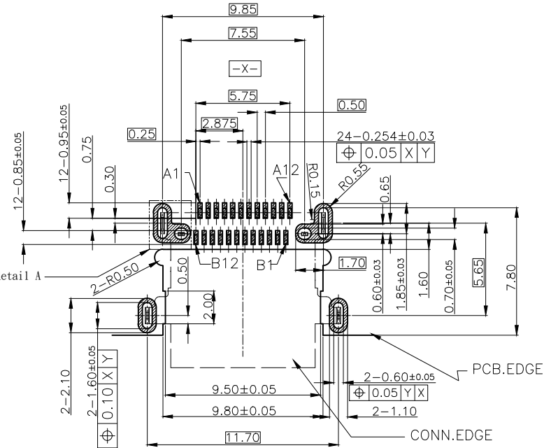
RECOMMENDED P.C.B LAYOUT(TOP VIEW) TOLERANCE= \pm 0.05 (THK:1.00mm)
