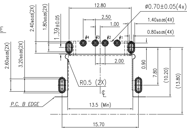
Recommended P.C.B Layout (THK:1.0mm) Top View (Tol:±0.05)
