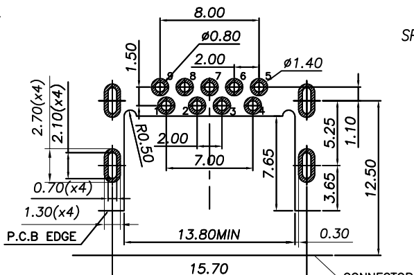
RECOMMENDED P.C.B PATTERN LAYOUT TOLERANCE ±0.05mm T=1.20±0.05
