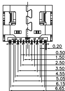
USB TYPE-C PIN ASSIGNMENTS
