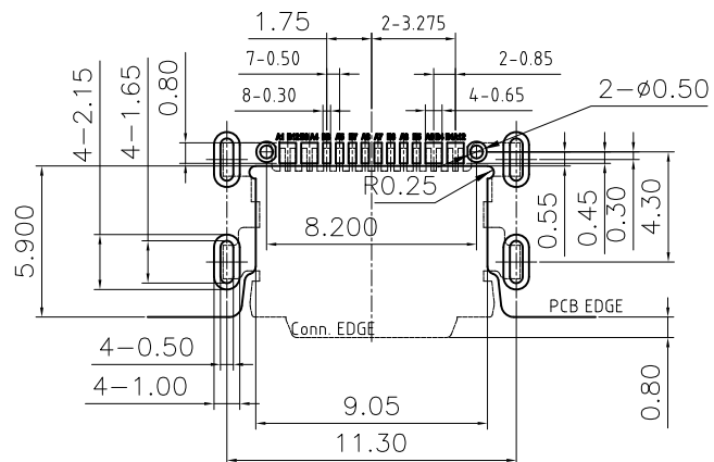
RECOMMENDED PCB LAYOUT TOLERANCE:±0.05 STENCIL THICKNESS:0.12mm
