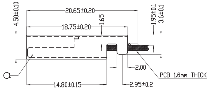
COMPONENT SIDE (PCB LAYOUT)
