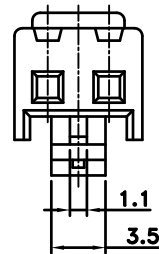
2Pin VIEW
