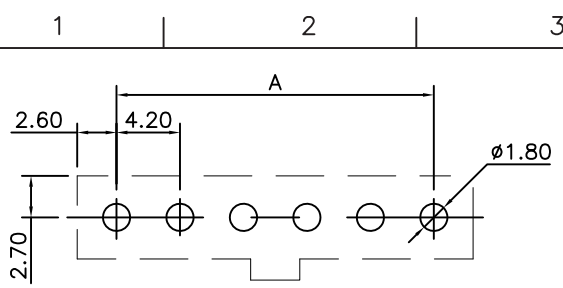
Recommended PCB Layout(Top View) General tolerance:±0.05mm
