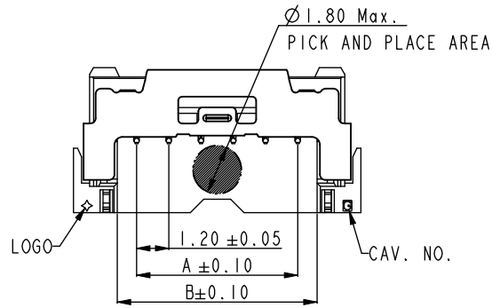
Shell Unlock Condition (REF.)
