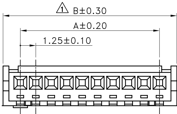
4~15 Circuit(Double Lock)
