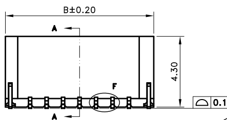
DETAIL F (SCALE 2:1)
