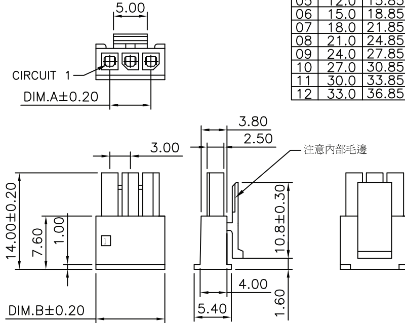
For 3-12 Pin
