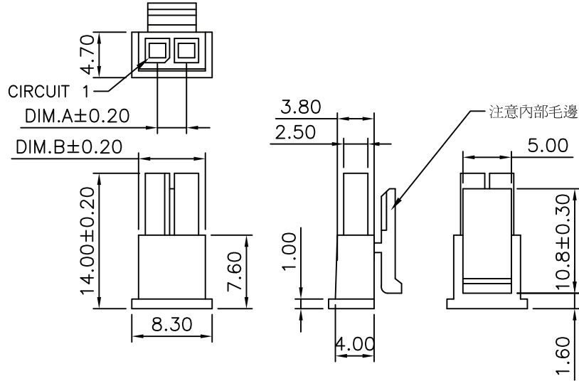
For 2 Pin
