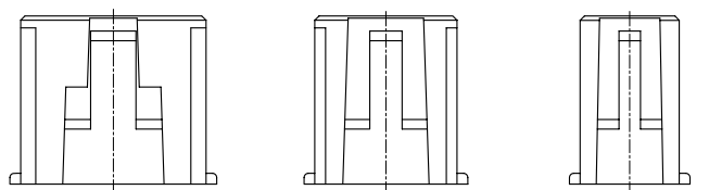
4~16Pin Circuit 3Pin Circuit 2Pin Circuit
