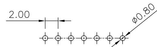
RECOMMENDED P.C.BOARD HOLE DIMM.
