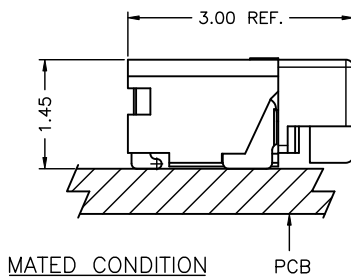
MATED CONDITION
