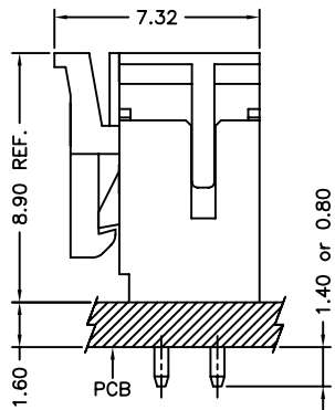
MATED CONDITION
