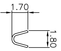
B-B SEC
