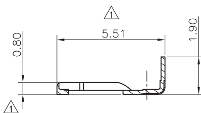
B-B SEC
