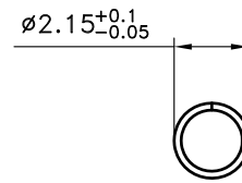
C-C SEC
