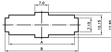
16~18 Circuit (Double Row)
