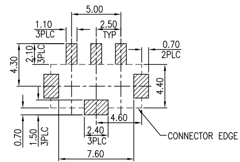
RECOMMENDED PC. BOARD LAYOUT (TOL.±0.05)(TOP VIEW)
