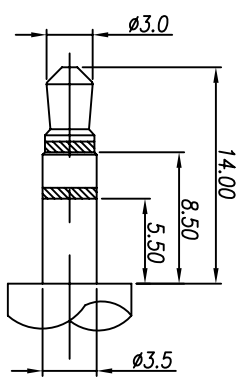
3.5 3 POLE STANDARD PLUG
