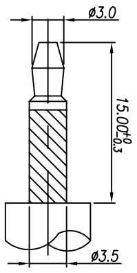
OPTICAL FIBER PLUG
