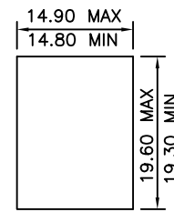
Single Panel-Latch Clearance Panel Thickness 1.60mm
